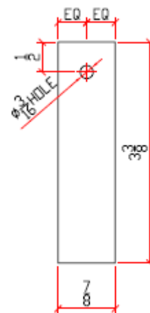
Cutout Dimensions: 3-3/8" L x 7/8" W x 3/4" D
